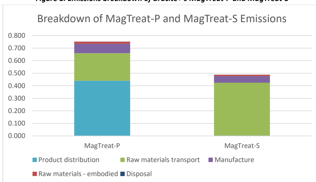
Figure 1: Emissions breakdown of Brucite+'s MagTreat-P and MagTreat-S
